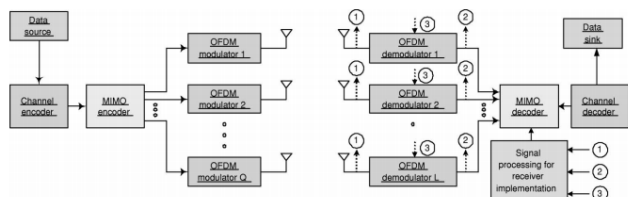
Fig. 5. MIMO-OFDM system model [15]
